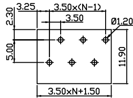
B type PCB LAYOUT
