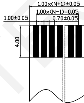
Proper Cable
