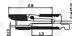
SECTION B-B SCALE 1:1
