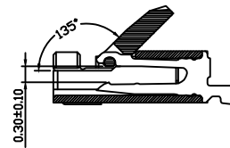
SECTION B-B SCALE 1:1 When Cover Is Opene
