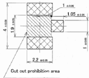
RECOMMENDED FOOTPRINT PATTERN
