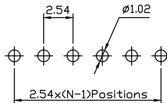
Recommended P.C.B Hole Layout
