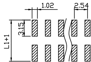
Recommended P.C.B Hole Layout
