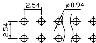
Recommended P.C.B Hole Layout
