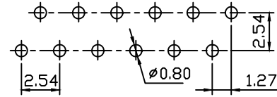
Recommended P.C.B Layout(Top Side) (PCB BOARD TOLERANCE±0.05)
