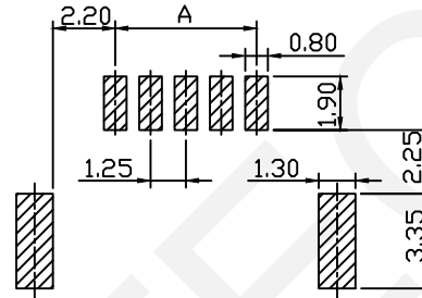
Recommended PCB Layout General Tolerance±0.1
