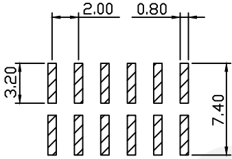
Recommended PCB Layout (Top Side) (PLB BOARD TOLERANCE ±0.05)
