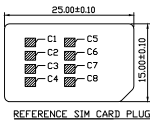
REFERENCE SIM CARD PLUG
