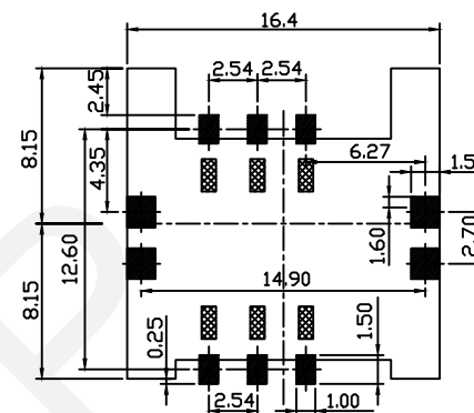
RECOMMENDED PCB LAYOUT TOP VIEW(XX±0.05)
