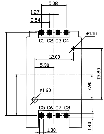
REFERENCE PCB LAYOUT UNIT:MM TOLERANCE:±0.05
