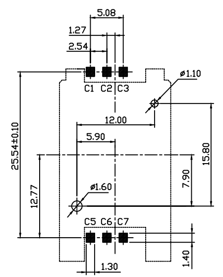
REFERENCE PCB LAYOUT UNIT:MM TOLERANCE:±0.05
