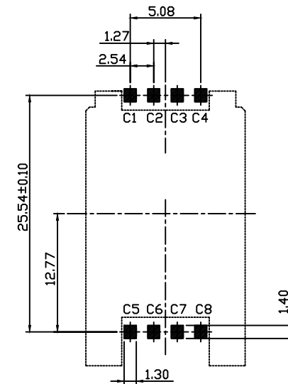
REFERENCE PCB LAYOUT UNIT:MM TOLERANCE:±0.05
