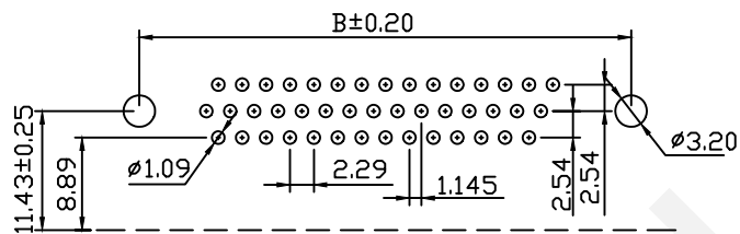
RECOMMENDED PCB LAYOUT TOLERANCE:±0.05mm
