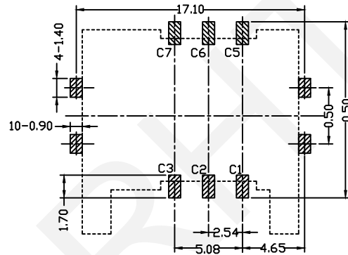
RECOMMENDED PCB MOUNTING PATTERN
