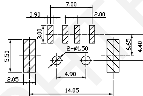
RECOMMENDED PCB LAYOUT TOLERANCE: ±0.05mm
