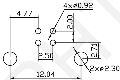
RELOMMENDED PCB LAYOUT
