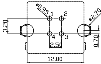
RECOMMENDED P.C.B.LAYOUT TOP VIEW(TOLRANCE:±0.05)
