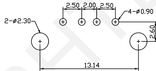
RECOMMENDED PCB LAYOUT TOLERANCE:±0.05mm
