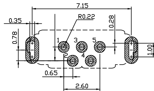
RECOMMENDED PCB LAYOUT THICKNESS:1.0mm
