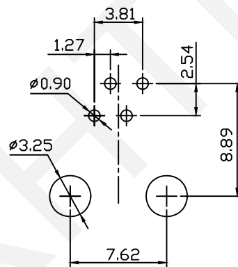
PCB Layout
