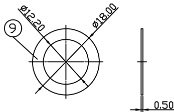
WASHER
