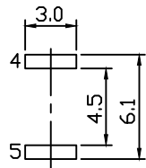
PCB LAYOUT TOP VIEW
