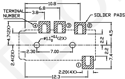
RECOMMENDED SOLDER PAD LAYOUT (TOP VIEW)
