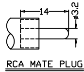
RCA MATE PLUG
