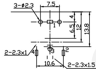
T1.6 Dimensions Of PCB Holes Tolerance: \pm 0.1 (Printed-Side View)
