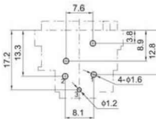
PCB LAYOUT (VIEWED FROM COPPER SIDE)
