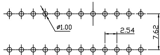
PCB Layout
